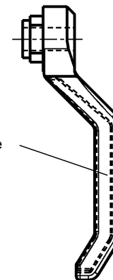
Handle short
