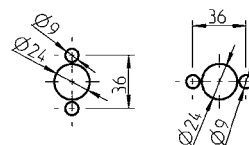
Cut out door version... LH RH
