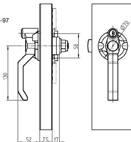
Cut out door version... LH RH
